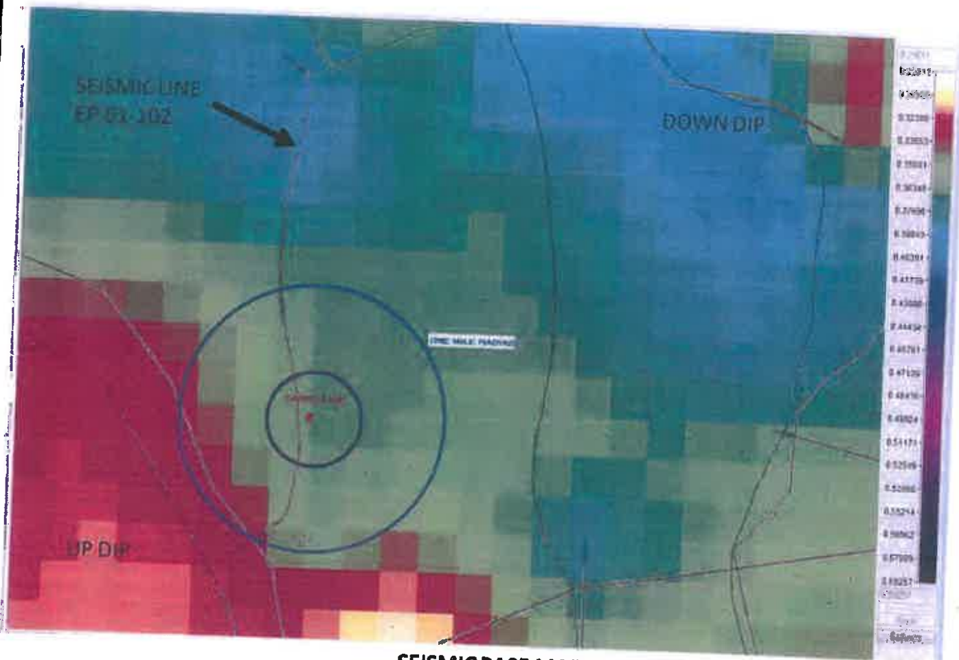
SEISMIC BASE MAP TOP INJUN TIME GENERATED FROM 2D SEISMIC LINES NO FAULTS FOUND WITHIN SHALLOW SECTION
